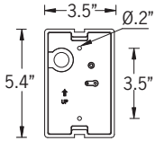
Mounting Detail
