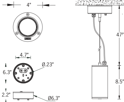
Mounting Detail
