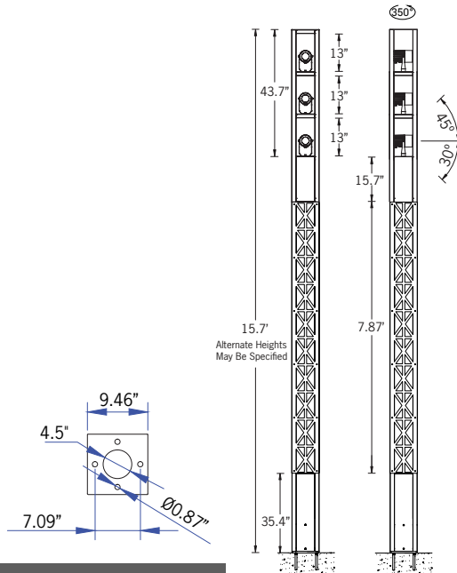
Mounting Detail
