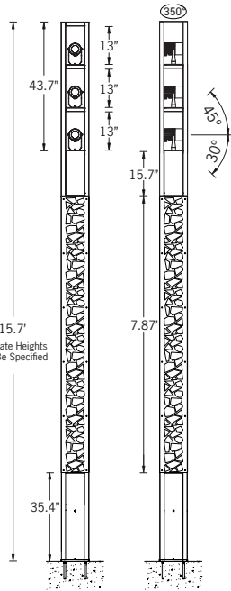
Mounting Detail
