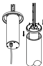
Standard Internal Waterproof Driver Housing
