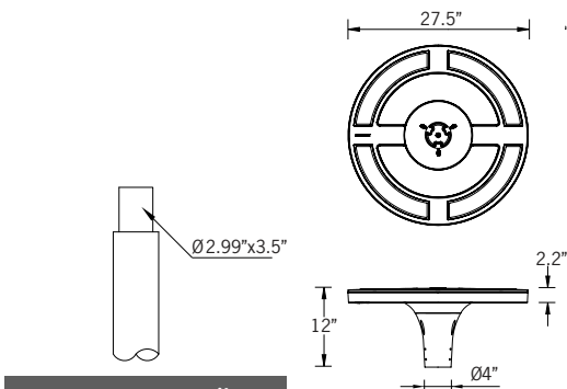
Tenon Detail
