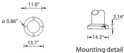
Mounting detail
