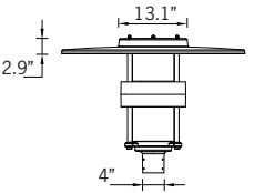
Fixture Detail
