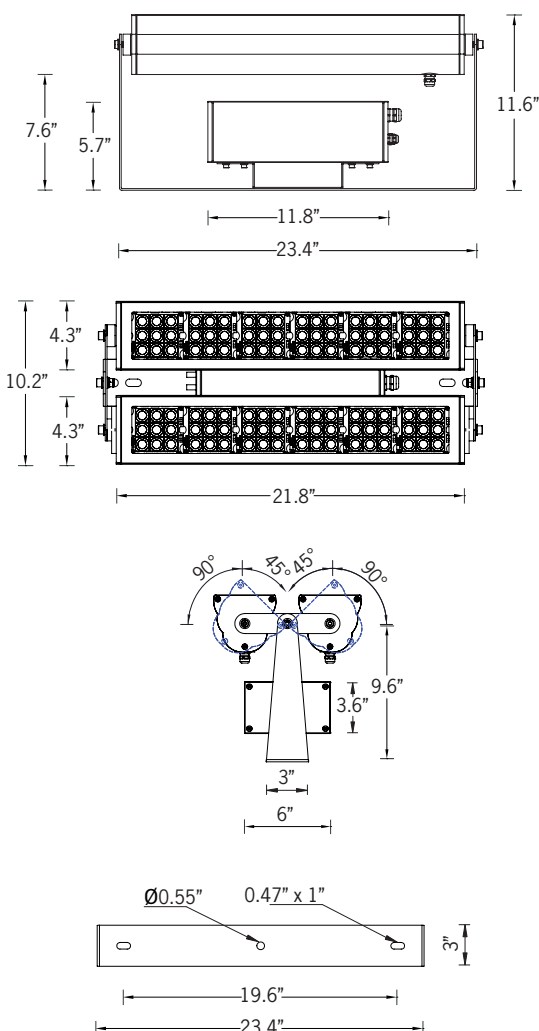
Mounting Detail
