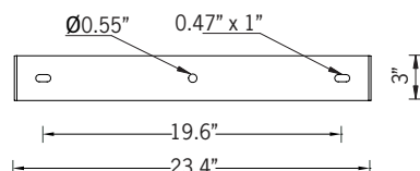
Mounting Detail
