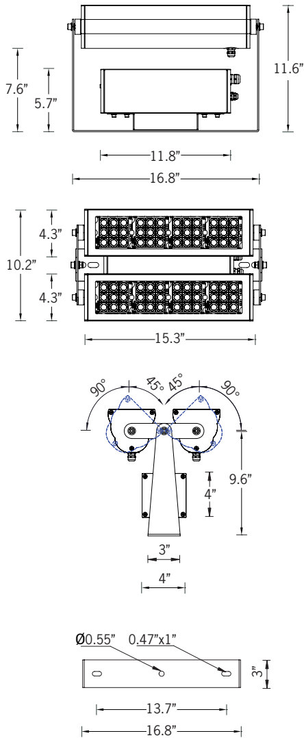
Mounting Detail
