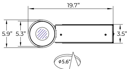
Ceiling Hole Size
