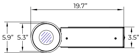
Ceiling Hole Size
