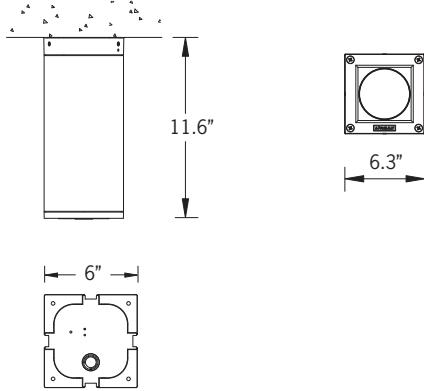
Mounting Detail
