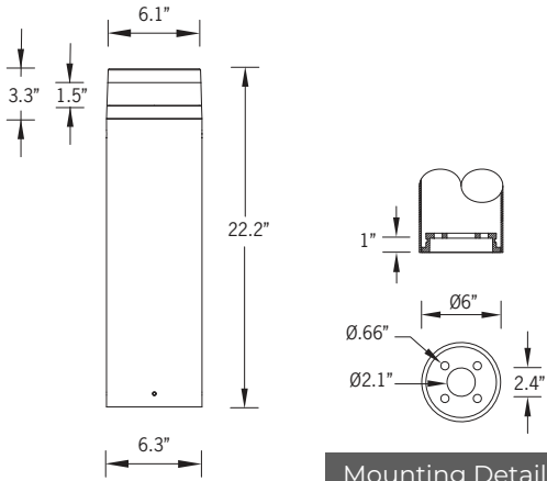
Mounting Detail
