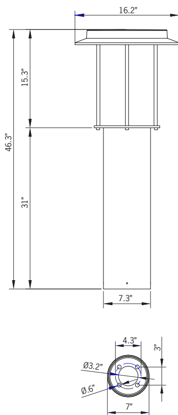
Mounting Detail
