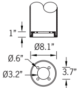
Mounting Detail
