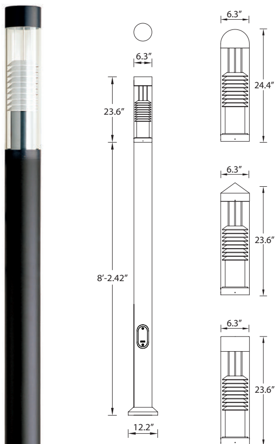
Mounting detail
