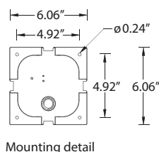
Mounting detail
