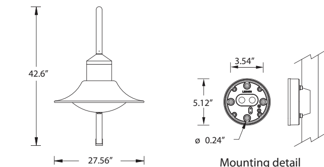
Mounting detail
