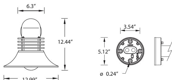
Mounting detail
