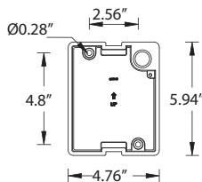
Mounting detail
