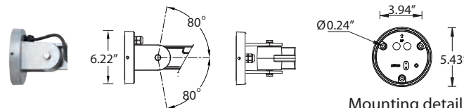
Mounting detail for adjustable arm
