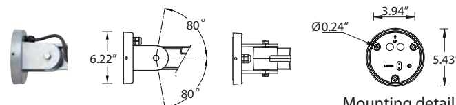
SAM - Small Adjustable Arm
