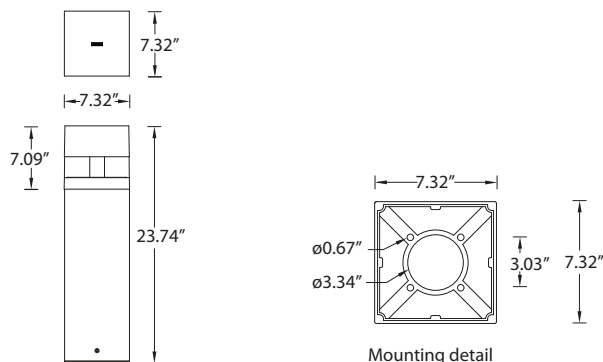
Mounting detail
