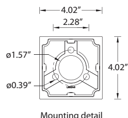
Mounting detail
