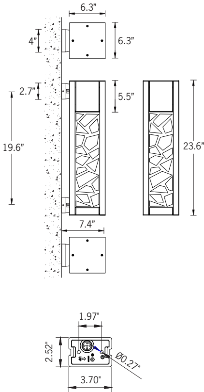
Mounting Detail
