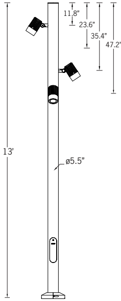
Floodlight Detail
