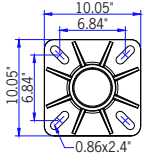
Mounting Detail
