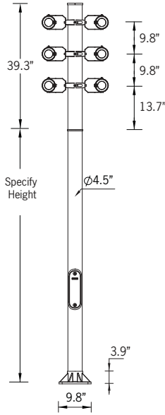
Mounting Detail
