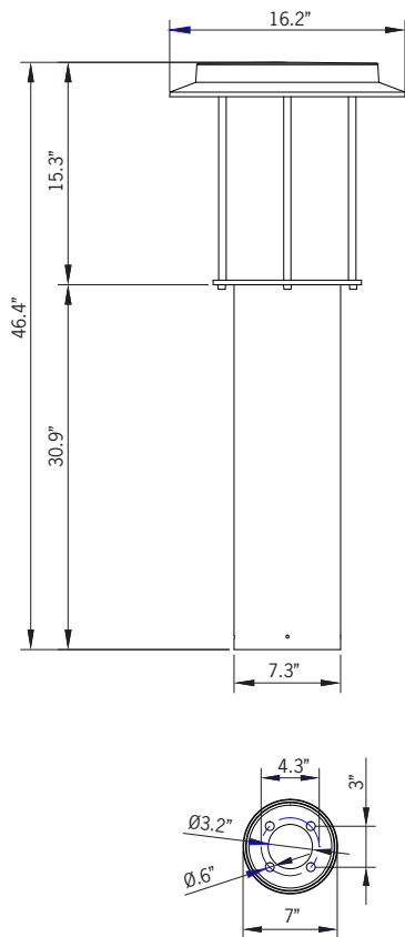
Mounting Detail
